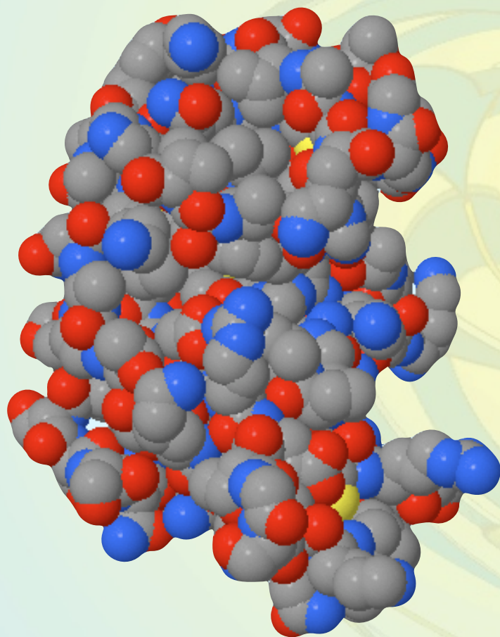
Ribonuclease A
