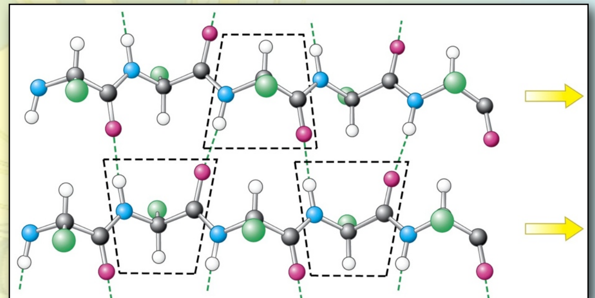
Parallel \beta -sheet
