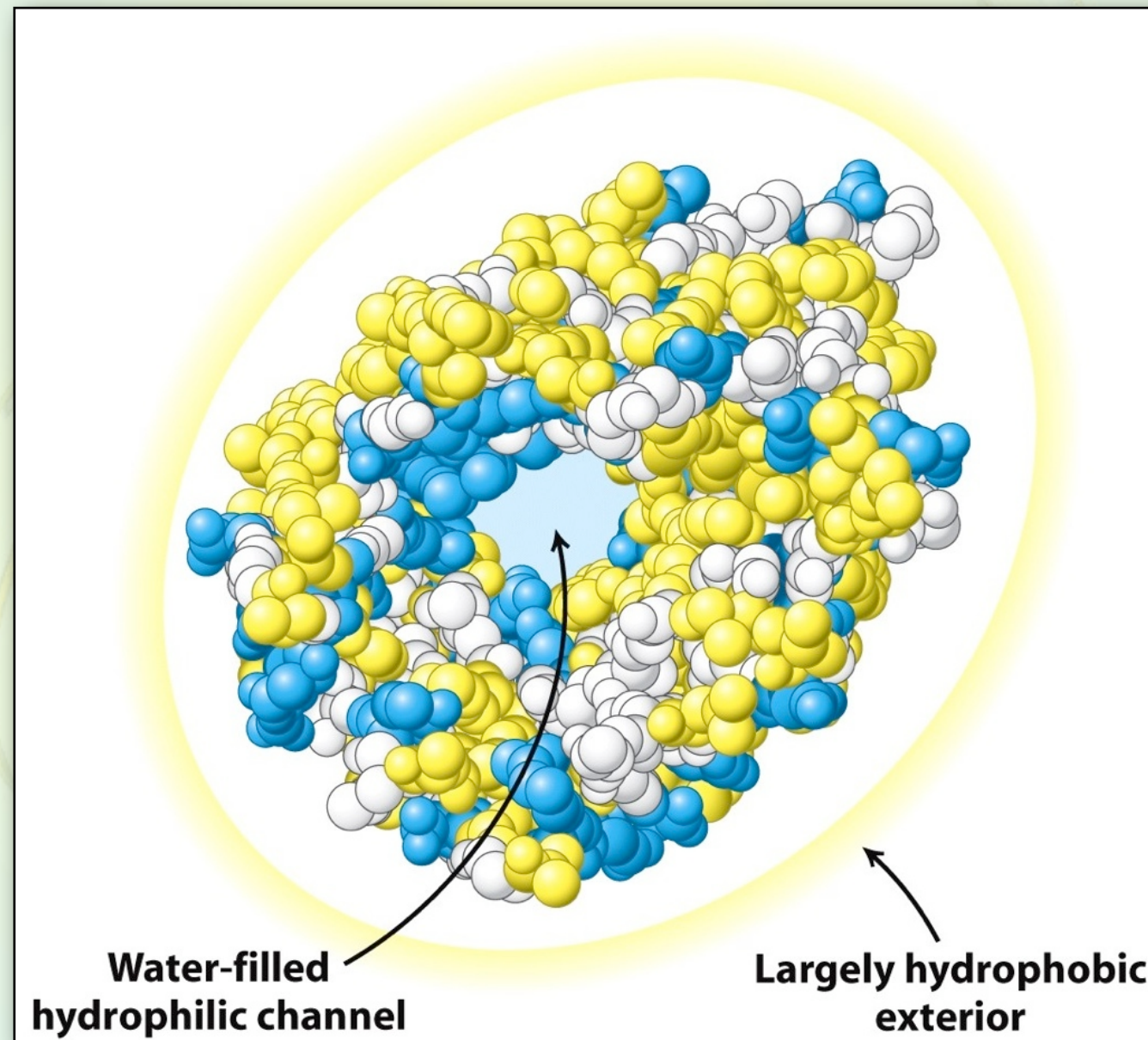
Porin, a membrane protein
