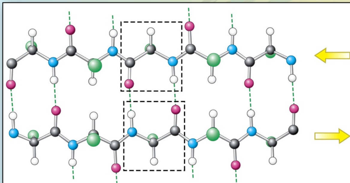
Antiparallel \beta -sheet
