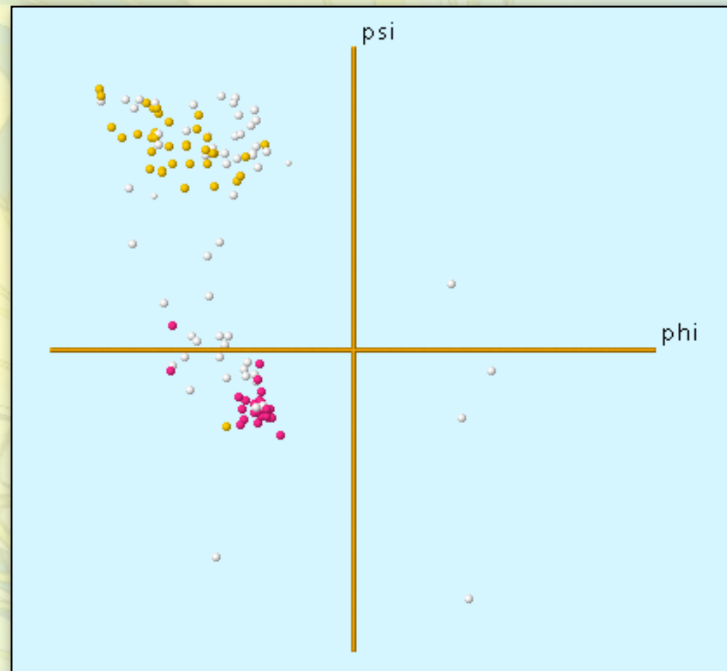
Ribonuclease A
