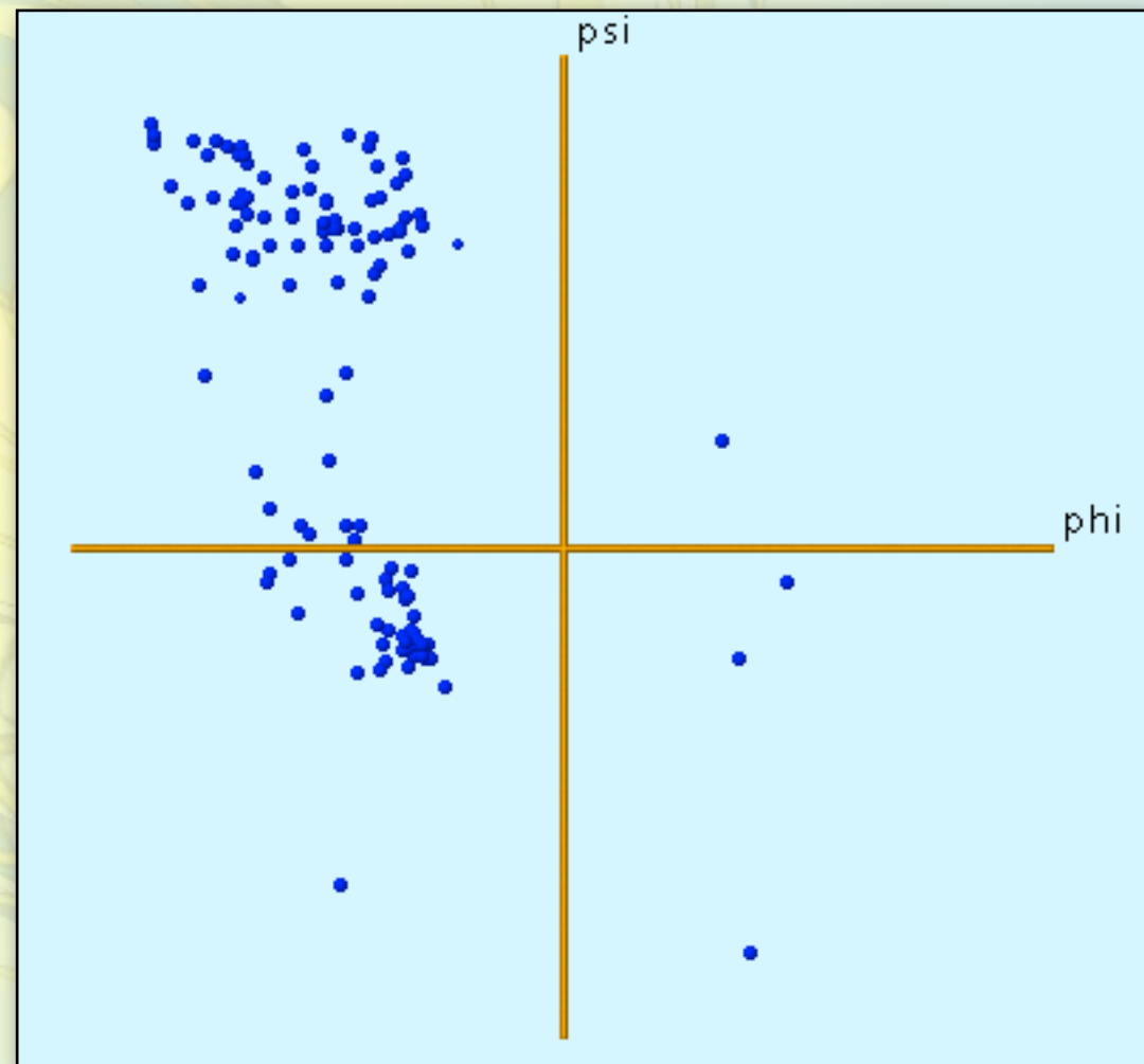
Ribonuclease A
