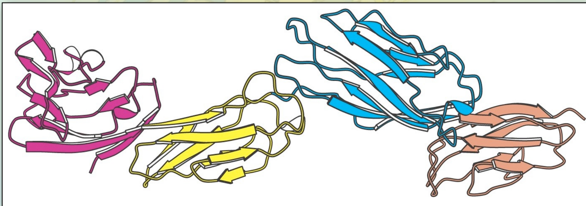
CD4 protein
