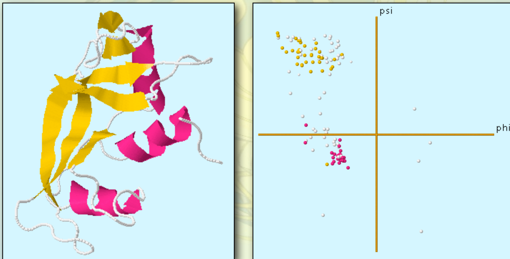
Ribonuclease A
