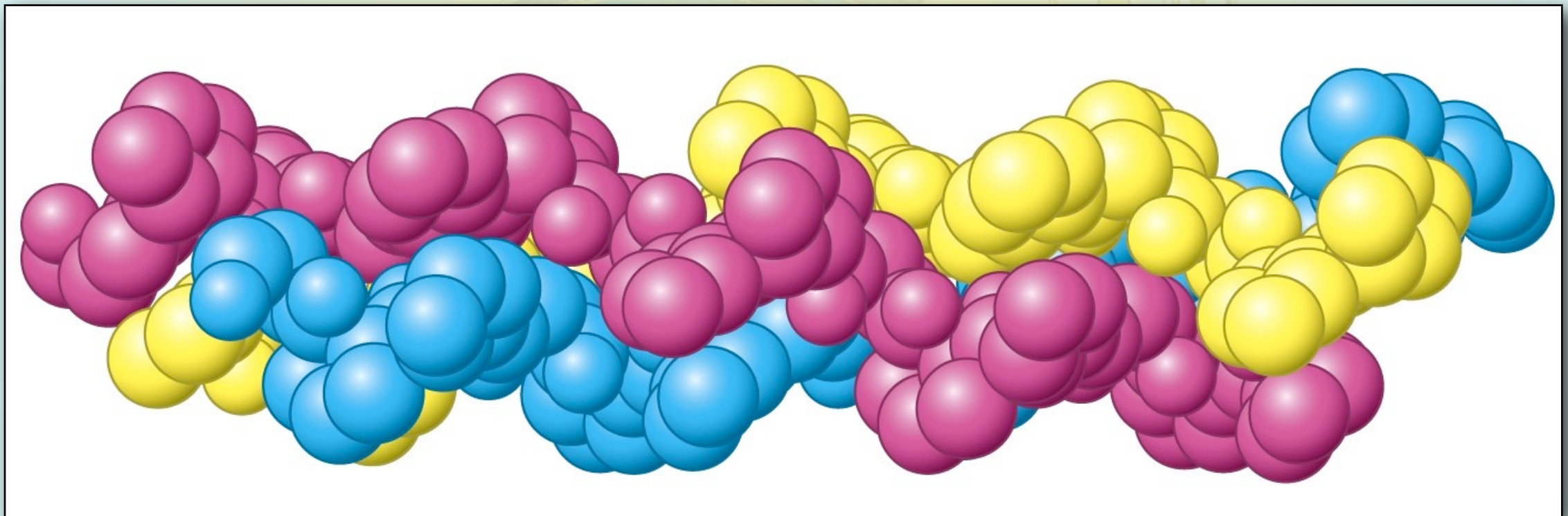
Collagen (polyproline triple helix)
