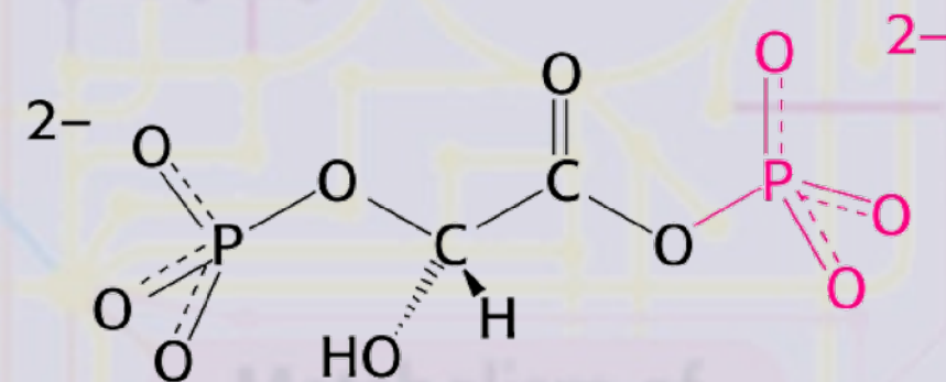
1,3-Bisphosphoglycerate
