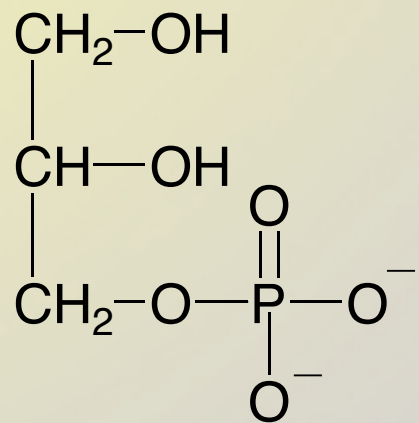
Glycerol 3-phosphate
