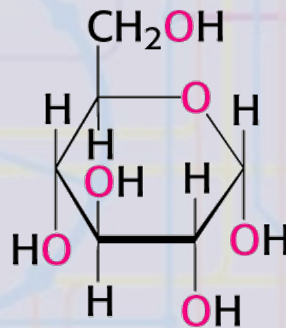
Glucose
