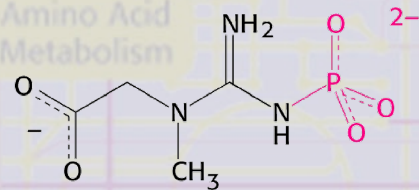
Creatine phosphate
