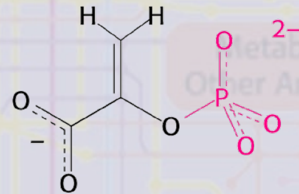
Phosphoenolpyruvate
