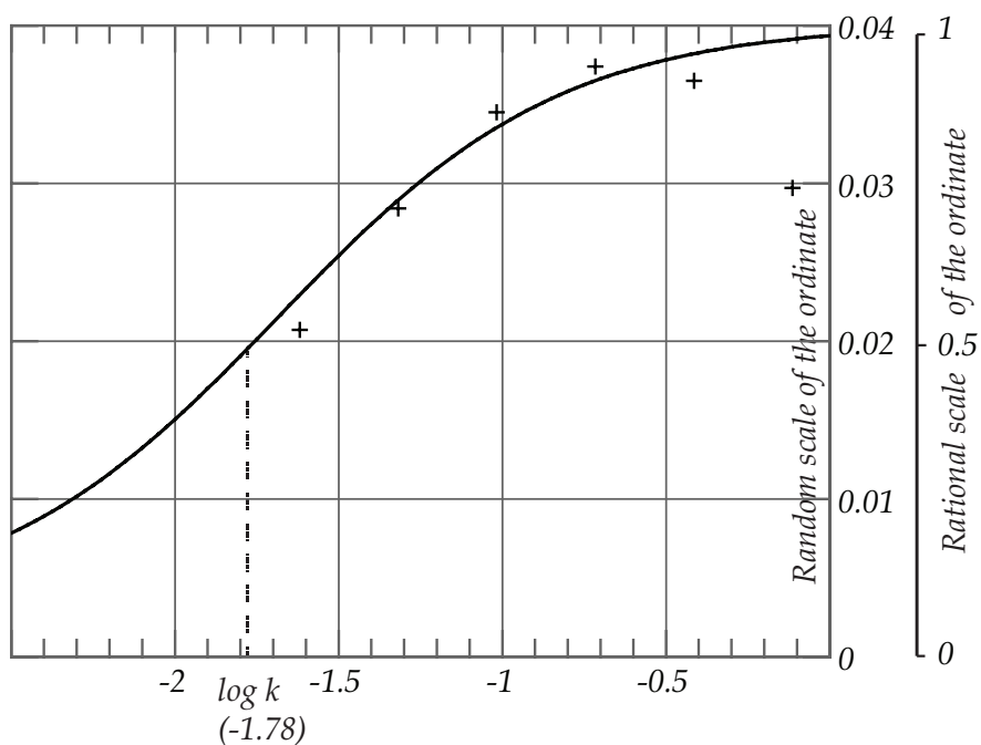
Fig 4a. Representation as Fig. 1a. Calculated from the experiment of Fig. 4.
