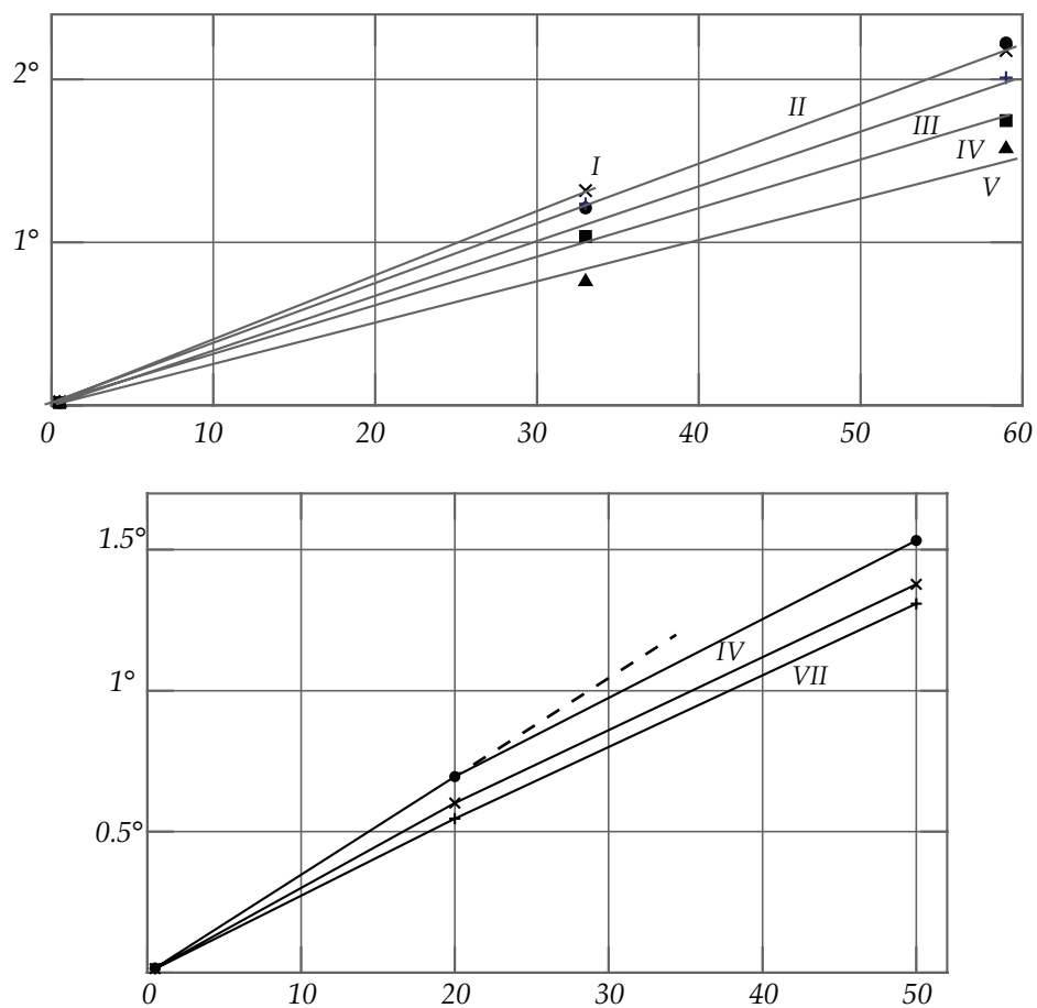
Fig. 13. (corresponding to Table 13) and Fig. 14 (corresponding to Table 14). Effect of mannose.
