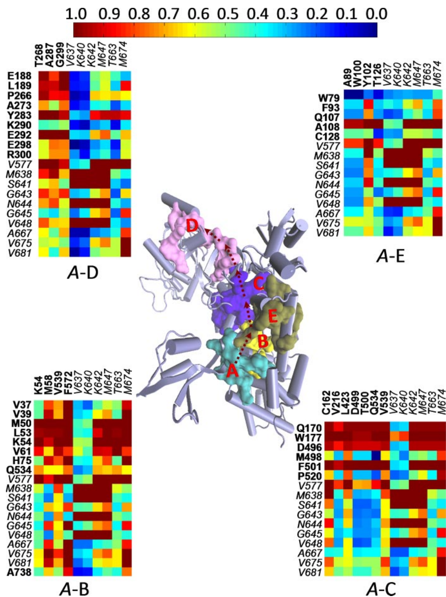
FIGURE 6. Trajectory of correlated motions observed through clusters of coevolving residues. The motion path is shown with broken-lined arrows. The five clusters (A–E) are mapped on to the Tt LeuRS structure and are displayed at the center. The four SCA plots showing both intra- and intercouplings between A with four other clusters are displayed at corners. Residue numbers shown in italics belong to Cluster A.
