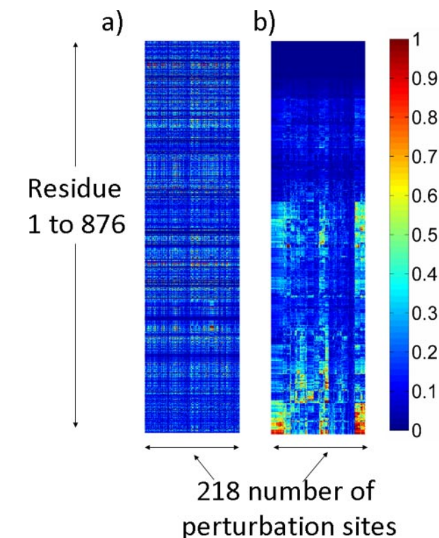
FIGURE 5. Statistical coupling analysis of the LeuRS family. Statistical coupling matrix: a , no clustering; b , one-dimensional hierarchical clustering showing the co-evolving residues. The color gradient, as indicated in the color bar, is as follows: blue squares represent the lowest ( 0 kT^* ), and red squares represent the highest ( 1 kT^* ) statistical coupling energies, \Delta \Delta G_{ij}^{\text{stat}} (calculated using Equation 11).
