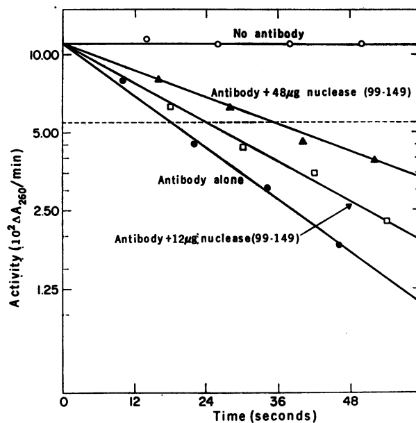
Fig. 12. Semilogarithmic plot of activity against time for assays of 0.05 \mu\text{g} of nuclease in the presence of: \circ — \circ , no antibody; \bullet — \bullet , 6 \mu\text{g} of antibody to (99 to 126) n ; \square — \square , 6 \mu\text{g} of antibody to (99 to 126) n plus 12 \mu\text{g} of (99 to 149); and \blacktriangle — \blacktriangle , 6 \mu\text{g} of antibody to (99 to 126) n plus 48 \mu\text{g} of (99 to 149). The dotted line represents one-half of the initial activity.
