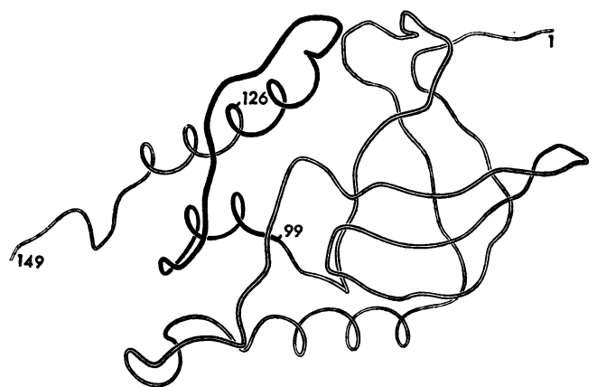
Fig. 7 (left). Amino acid residues in the sequence of nuclease that are of particular importance in the catalytic activity and binding of substrate and calcium ions (36). Fig. 8 (right). A schematic view of the three-dimensional structure of staphylococcal nuclease (31, 47).
